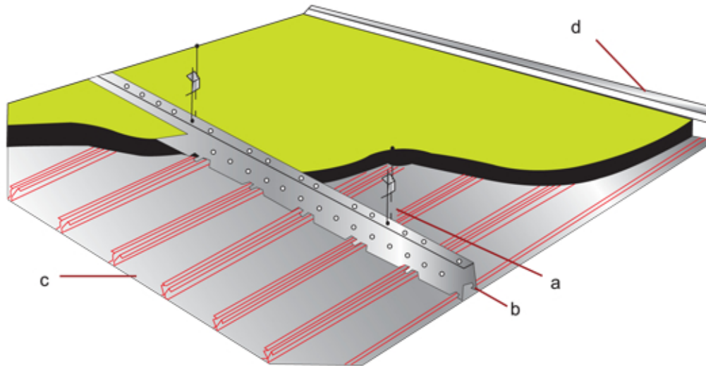
a. Adjustable suspension b. Carrier c. Strip plate d. Edge Cover
